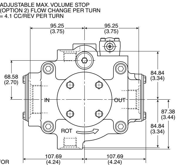
Rear View
